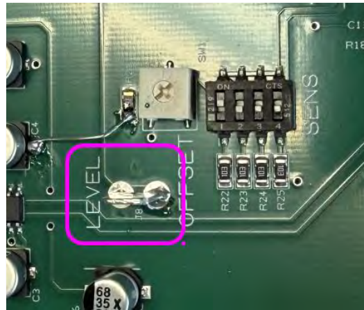
Figure 13, Monitoring detected Voltage Level
