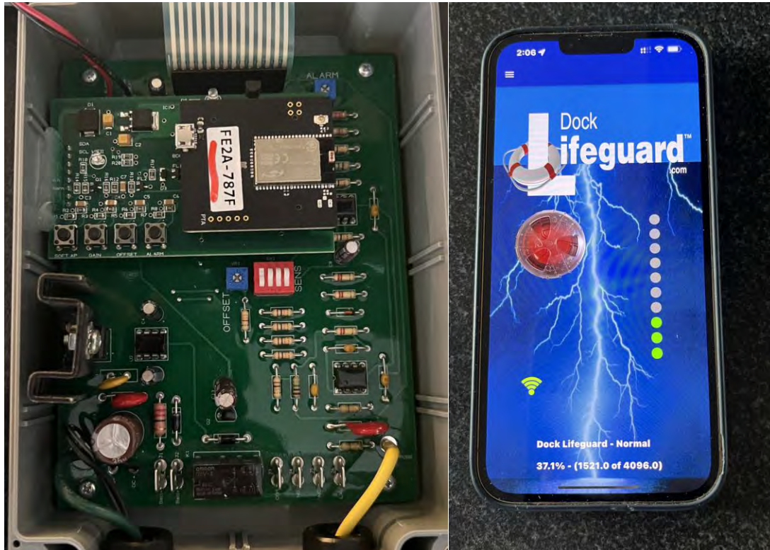
Figure 12, iOT Board for Push Notifications
