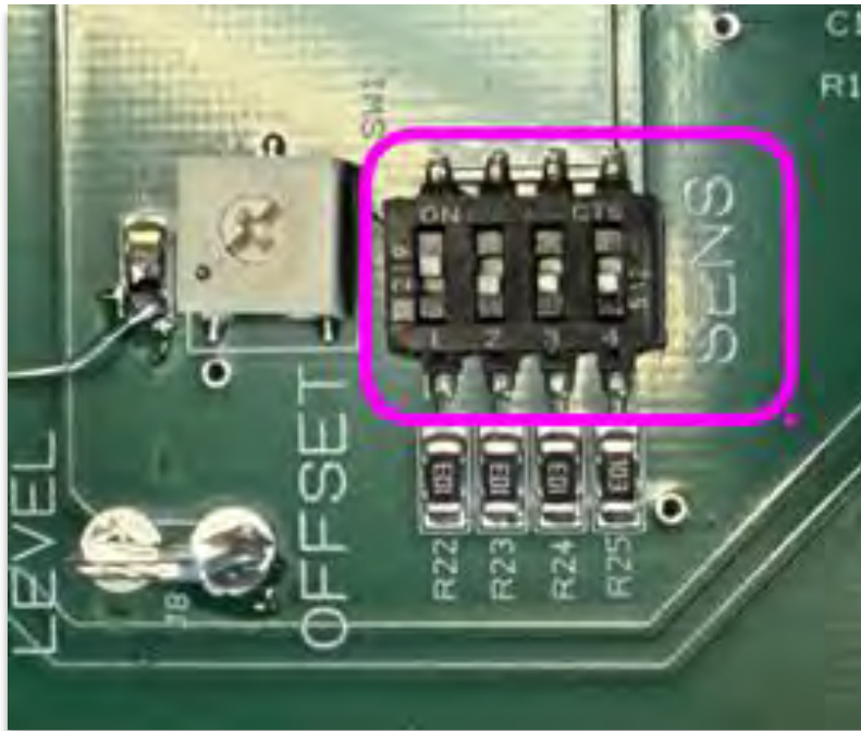
Figure 8, Sensitivity Dip Switch Block
