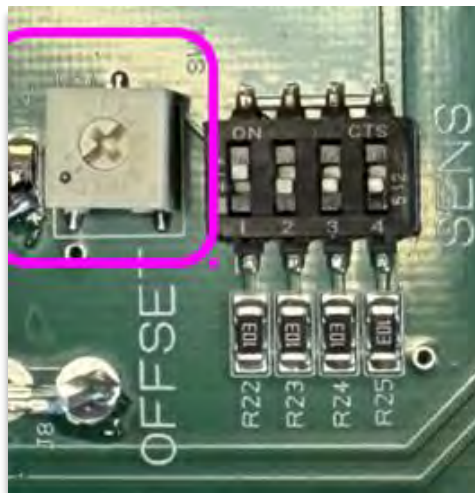
Figure 9, Zero Reference Point Potentiometer
