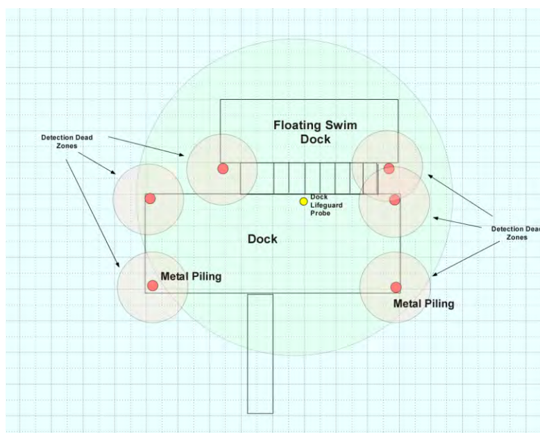
Figure 4, Steel Piling Dock
