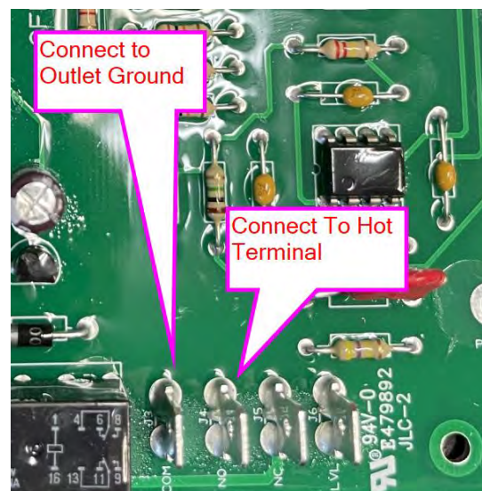
Figure 14, GFCI Trip Wire, 2307xxxx Serial Numbers
