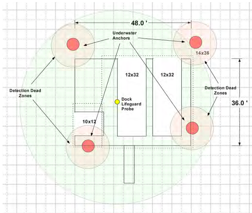
Figure 3, Floating Dock with Underwater Anchors
